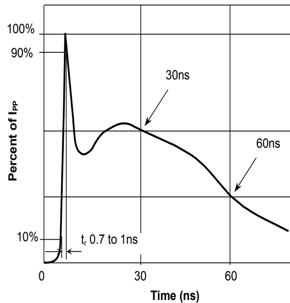
Fig.4 Pulse Waveform-ESD(IEC61000-4-2)
