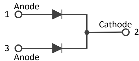
TO-220AB
