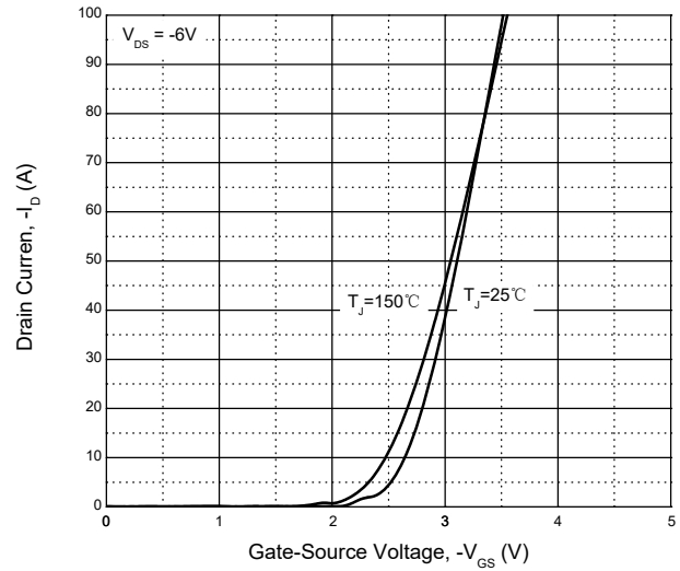
Fig. 2 - Transfer Characteristics
