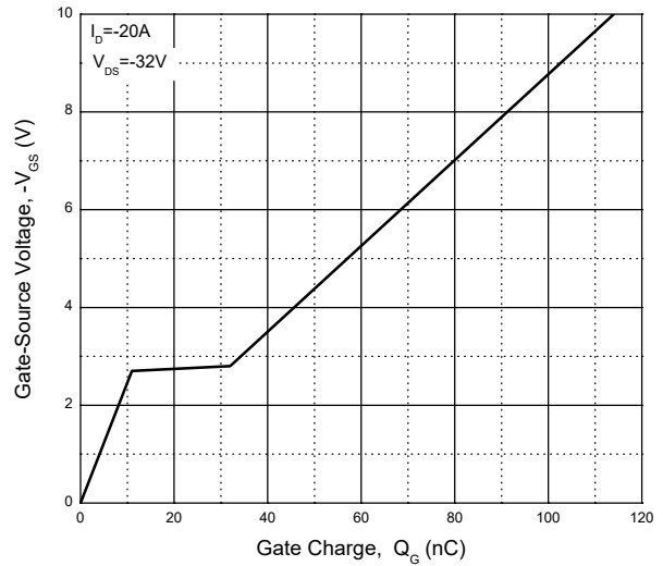
Fig. 8 - Gate Charge
