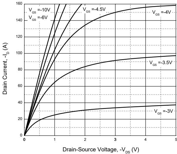
Fig. 1 - Output Characteristics
