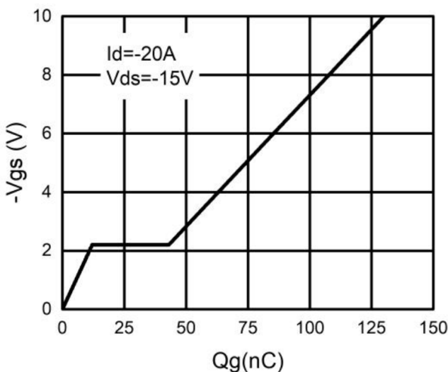
Fig.5 - Gate charge
