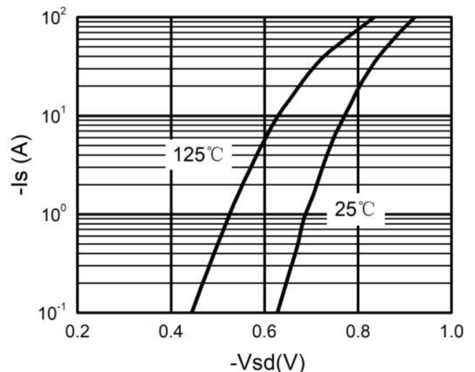
Fig.6 - Forward Characteristic
