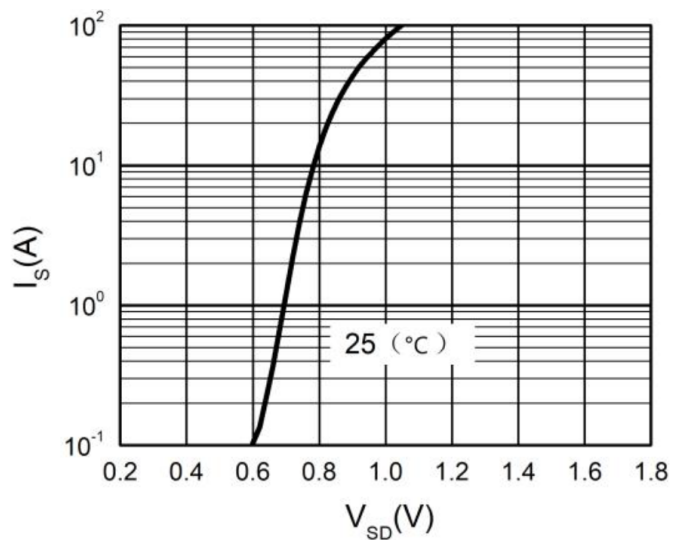
Fig.6 - Forward Characteristic
