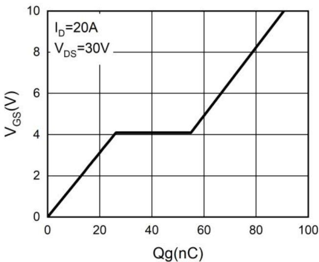
Fig.5 - Gate charge
