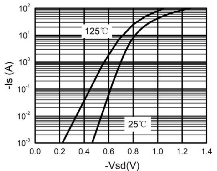
Fig.6 - Forward Characteristic
