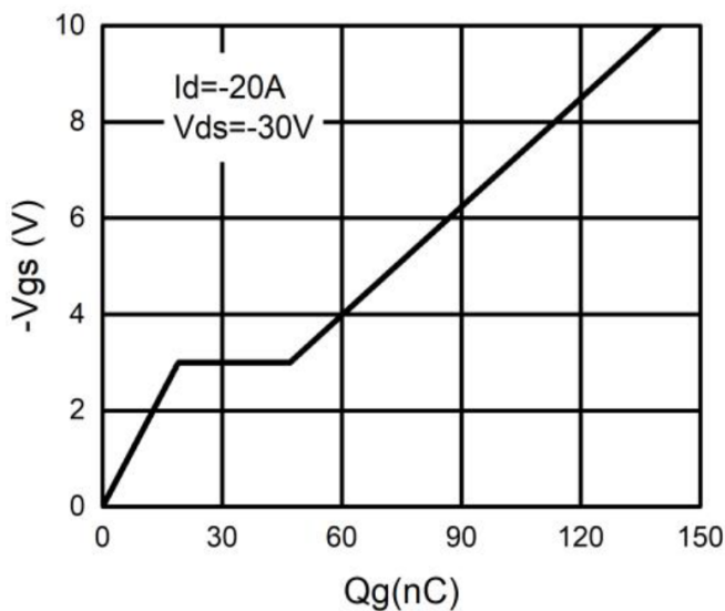
Fig.5 - Gate charge
