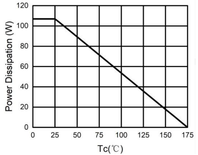
Fig.8 - Power Derating
