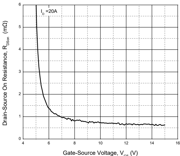
Fig. 5 - Drain-Source On-Resistance
