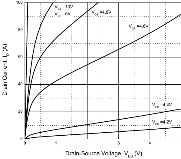
Fig. 1 - Output Characteristics
